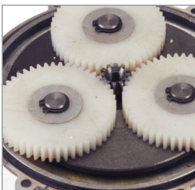
150/230 RPM Gear Box
